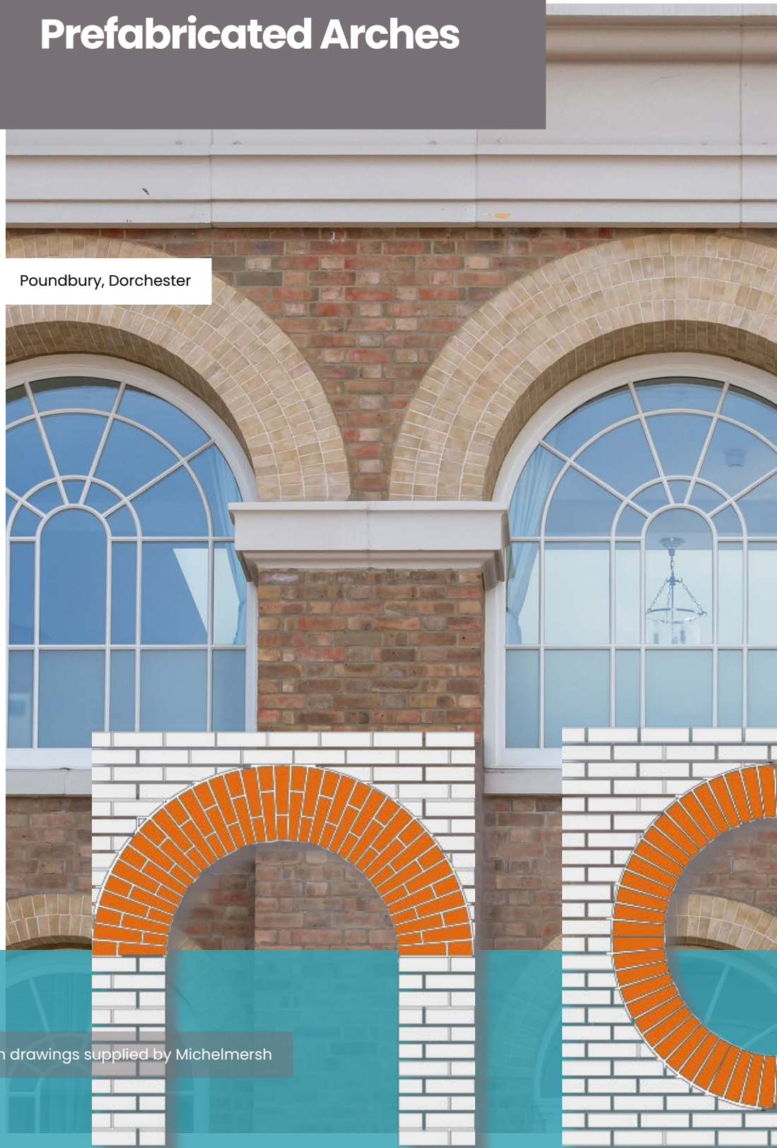
290mm High Semi-Circular Arch
