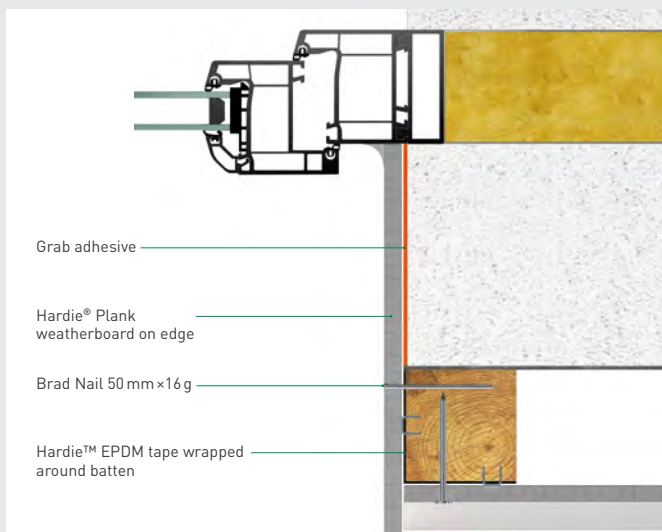
Window Reveal
