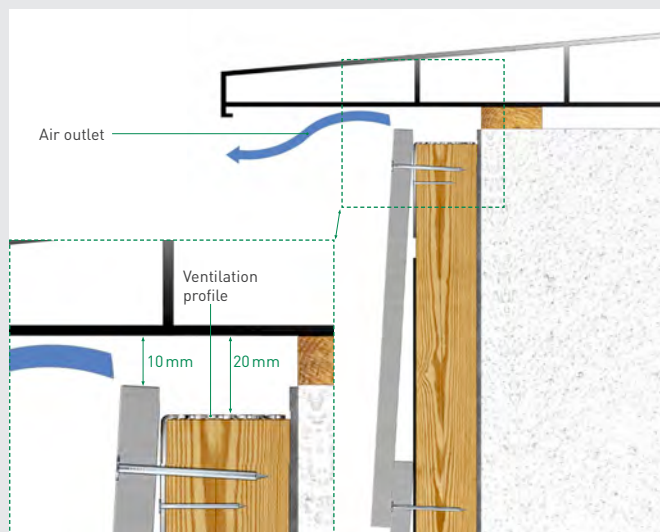
Window Cill
