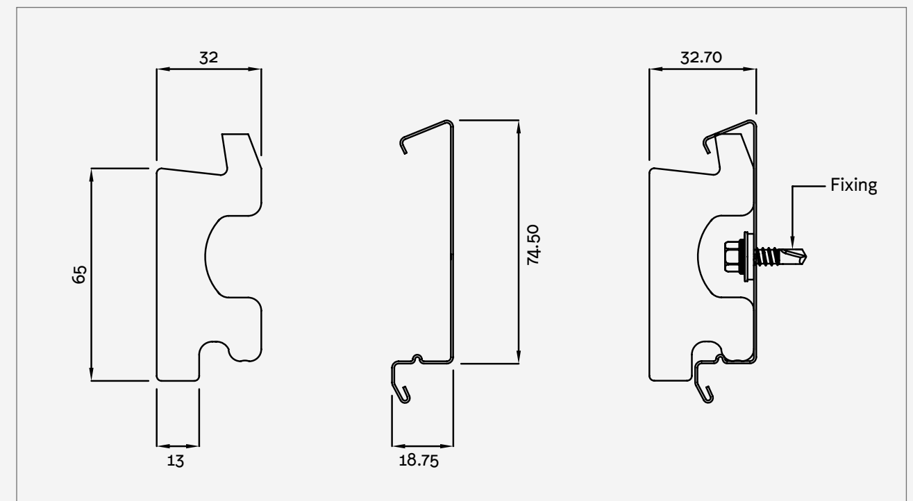
Corium Tile & Steel Backing Profile (Dimensions in mm)
