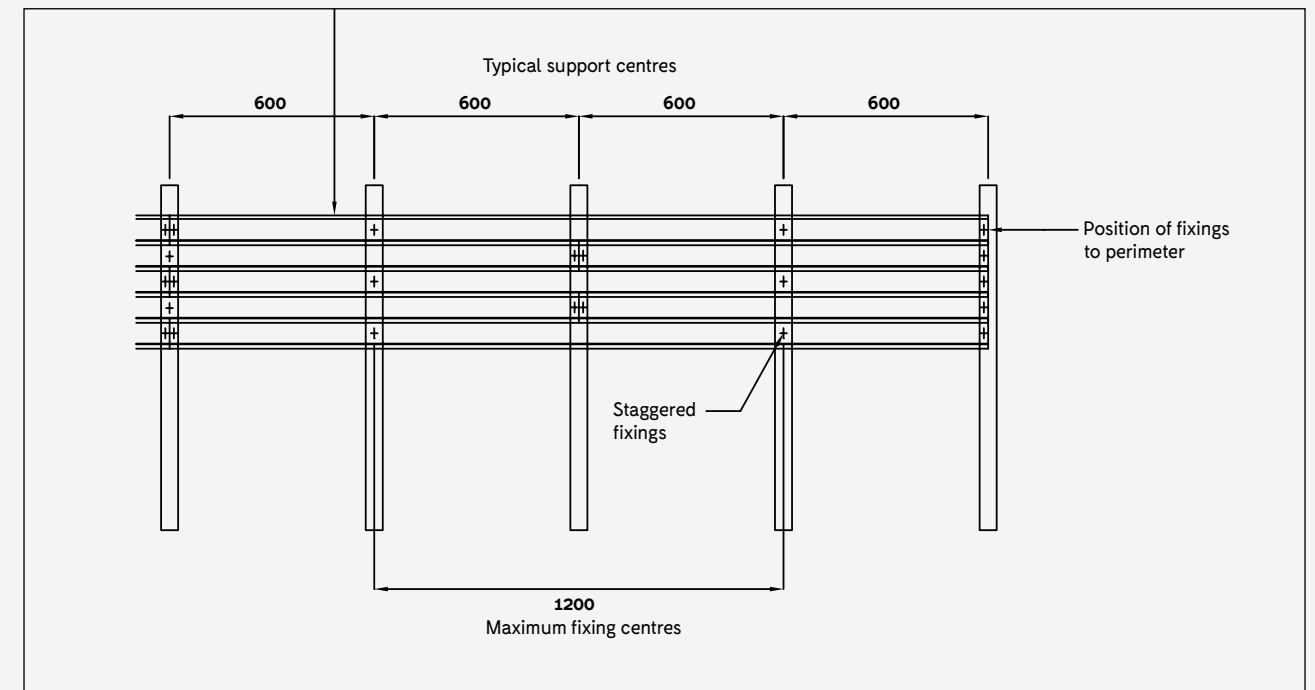
Typical fixing pattern of the Corium Brick Tile Cladding System
